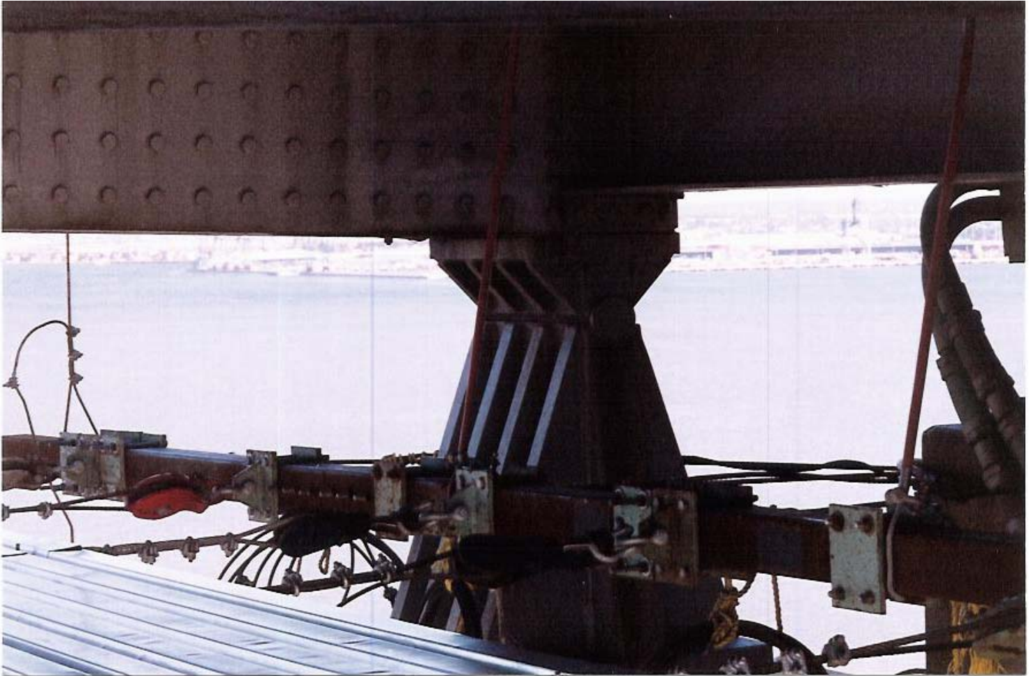
Lower Cable Supported/Metal Deck Platform & Horizontal Support Beam Assembly End Connection
